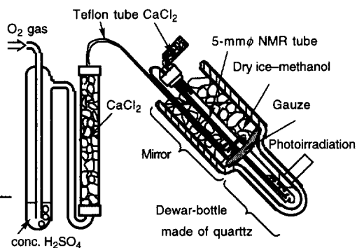
Fig. 3. An apparatus for low-temperature photooxygenation.
