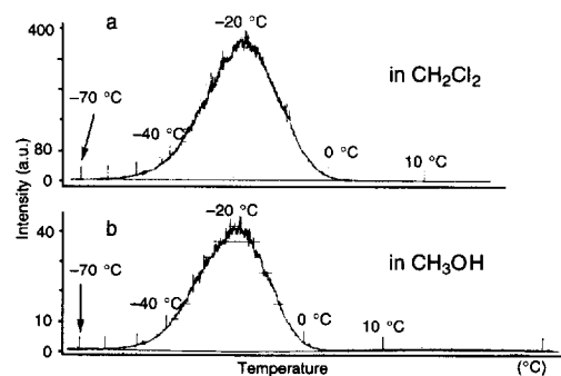
Fig. 18. Luminescence chart in cold solution while warming to room temperature. a: diluted with \text{CH}_2\text{Cl}_2 . b: diluted with MeOH. Photooxygenation: 10 min in \text{CF}_3\text{CH}_2\text{OH}-\text{CH}_3\text{OH} .
