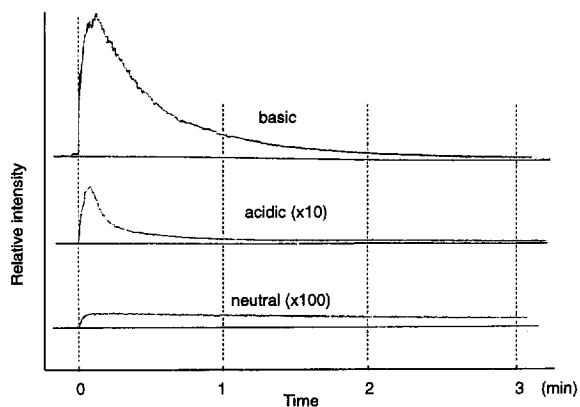
Fig. 14. Chemiluminescence chart of 1 in basic (containing 0.5 vol% of 0.25 M t -BuOK/ t -BuOH), acidic (containing 0.5 vol% of 0.2 M acetate buffer pH 5.6) or neutral (no additive) DGM. Concentration: 1 \times 10^{-6} M. Volume: 1.0 mL. Temperature: 23 °C.
