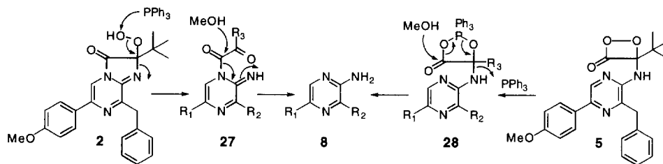
Scheme 5. Possible mechanism of the peroxides, 2 and 5 with triphenylphosphine to form aminopyrazine 8 .
