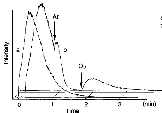
Fig. 2. Chemiluminescence chart of 1 in basic DGM. DGM was saturated with O 2 gas before 1 was added. a: spontaneous chemiluminescence initiated by adding 1 into DGM.
