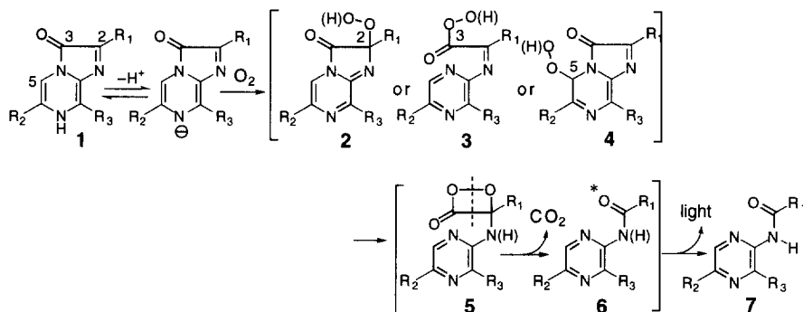
Scheme 1. Postulated luminescent mechanism and examples of coelenterate luciferin with imidazo[1,2-a]pyrazin-3-one system.
