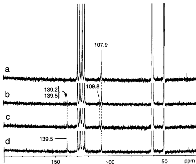
Figure 11. ^{13}\text{C} NMR spectra of low-temperature photooxygenation of 1(5\text{-}^{13}\text{C}) .
