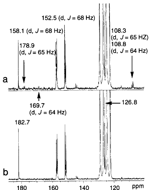
Fig. 12. ^{13}\text{C} NMR spectra of photo-products of 1(2,3\text{-}^{13}\text{C}_2) . a: after 10-min photooxygenation. b: after warming.
