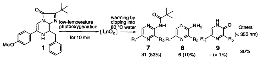
Scheme 3. Product determination in low-temperature photooxygenation. \text{LnO}_2 means the peroxidic luminescent intermediate. Yields in parentheses mean the corrected yield based on consumed 1 . Determination was carried out by HPLC with detection at 350 nm. ( \text{R}_1 = \text{C}_6\text{H}_4\text{OMe} , \text{R}_2 = \text{CH}_2\text{Ph} )
