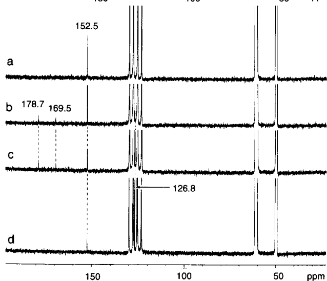
Fig. 10. ^{13}\text{C} NMR spectra of low-temperature photooxygenation of 1(3\text{-}^{13}\text{C}) .
