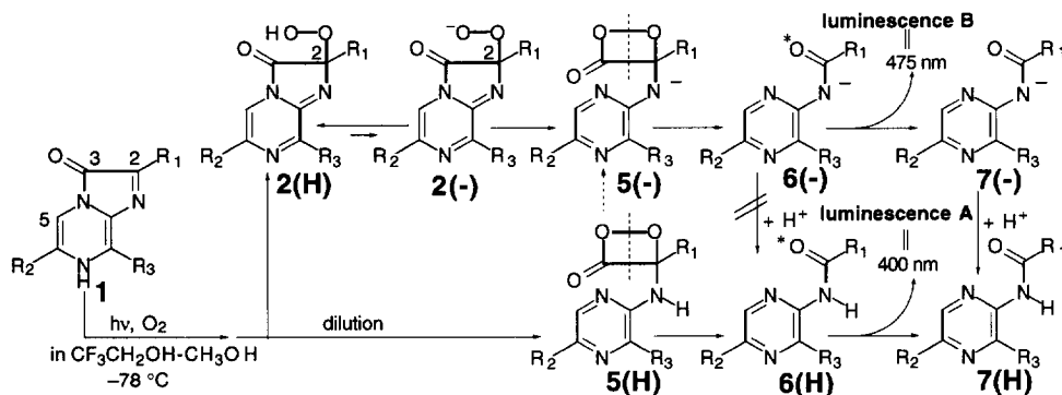
Scheme 6. Luminescence mechanism of two peroxides in neutral, acidic (pH 5.6) or basic DGM. The dotted arrow ( 5b to 5a ) indicates a possible pathway in basic DGM. ( R_1 = \textit{tert} -butyl, R_2 = \textit{p} -methoxyphenyl, and R_3 = \textit{benzyl} ).
