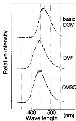
Fig. 1. Chemiluminescence spectra of 1 . Concentration: 3 \times 10^{-5} M. Basic DGM: see Fig. 15 caption.
