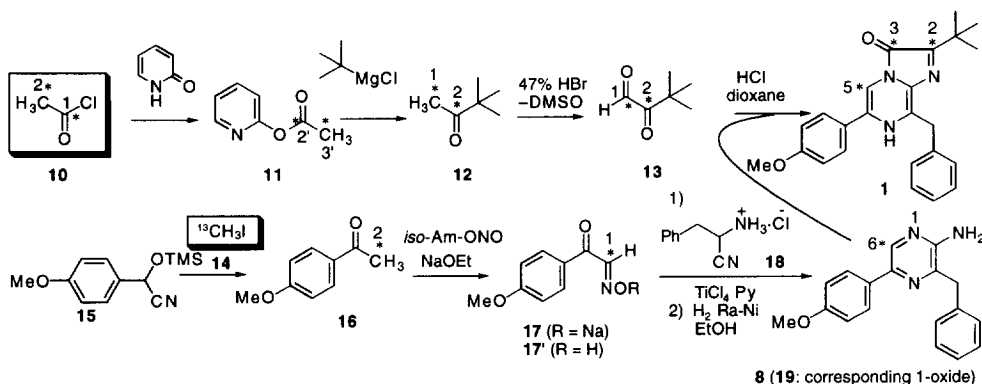
Scheme 2. Synthetic route of ^{13}\text{C} -enriched coelenterate luciferin analogs
