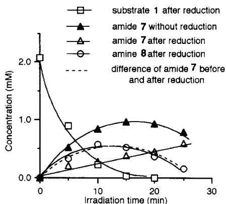
Fig. 7. Time course of low-temperature photooxygenation of 1 in \text{CF}_3\text{CH}_2\text{OH}-\text{CH}_3\text{OH} followed by \text{PPh}_3 reduction.
