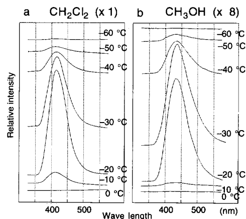
Fig. 19. Luminescence spectra in cold solution while warming to room temperature. a: diluted with \text{CH}_2\text{Cl}_2 . b: diluted with MeOH. Photooxygenation: 10 min in \text{CF}_3\text{CH}_2\text{OH}-\text{CH}_3\text{OH} .
