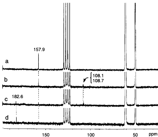
Fig. 9. ^{13}\text{C} NMR spectra of low-temperature photooxygenation of 1(2\text{-}^{13}\text{C}) .
