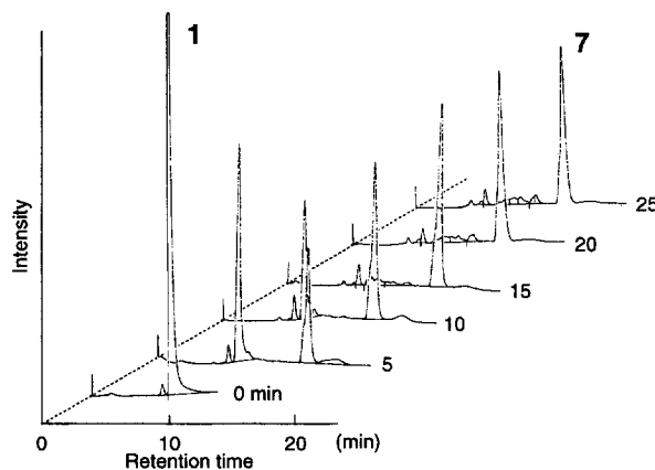
Fig. 4. HPLC chart of products in low-temperature photooxygenation of 1 in CF 3 CH 2 OH-MeOH (7:3). Mobile phase: MeCN-water (8:2) containing 0.1 vol% of TFA. Detection: UV 350 nm.
