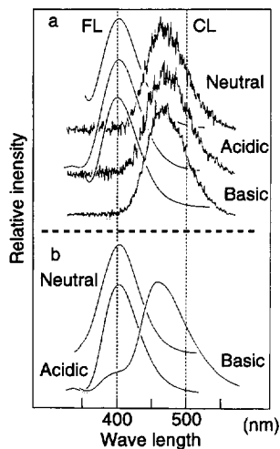
Fig. 13. Chemiluminescence and fluorescence spectra a: chemiluminescence spectra (CL) of 1 and fluorescence spectra of the spent solution after luminescence (FL) in neutral, acidic (pH 5.6) or basic DGM. b: fluorescence spectra of 7.
