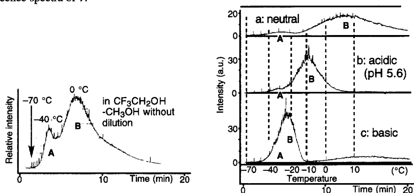
Fig. 15. Luminescence chart in cold DGM diluted solution while being allowed to come to room temperature. a: neutral DGM (no additives). b: acidic (pH 5.6) DGM (containing 0.5 vol% of 0.2 M acetate buffer of pH 5.6). c: basic DGM (containing 0.5 vol% of 1 M t -BuOK/ t -BuOH).
