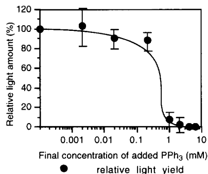
Fig. 8. Titration of the photooxygenated solution with \text{PPh}_3 . Photooxygenation time: 10 min.
