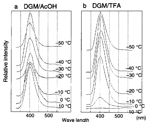
Fig. 17. Luminescence spectra in cold acidic DGM diluted solution while warming to room temperature.
