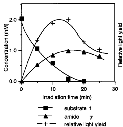
Fig. 5. Time course of photooxygenation of 1 in CF 3 CH 2 OH-CH 3 OH at -78 °C.
