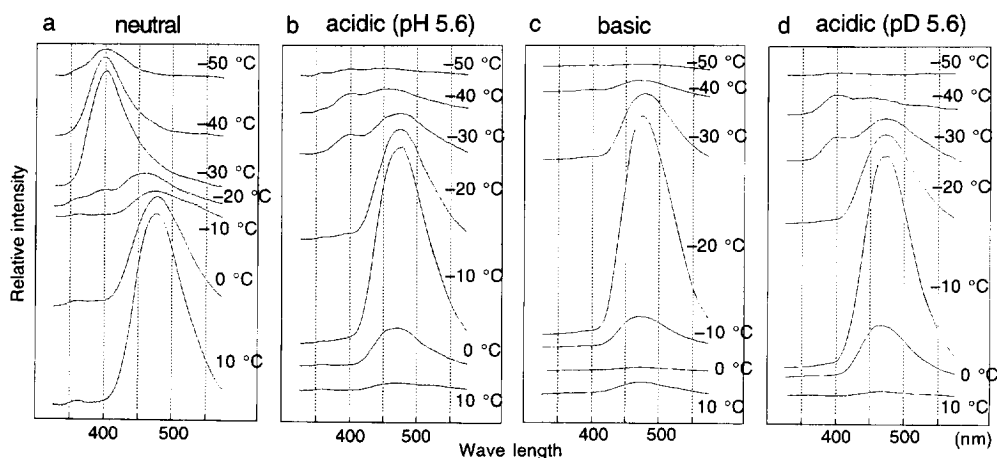
Fig. 16. Luminescence spectra of the diluted solution when allowed to come to room temperature. Neutral, acidic (pH 5.6) or basic: see Fig. 15 caption.
