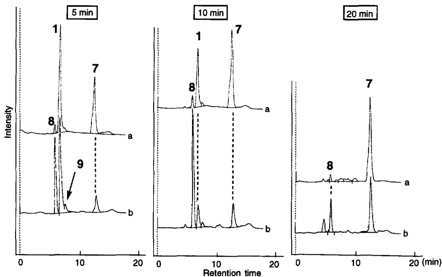
Fig. 6. HPLC chart of products in low-temperature photooxygenation in \text{CF}_3\text{CH}_2\text{OH}-\text{CH}_3\text{OH} (7:3). a: without reduction. b: after reduction with \text{PPh}_3 .
