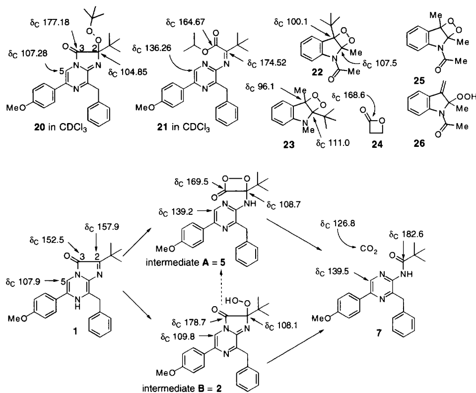
Scheme 4. Possible assignment of products in photooxygenation
